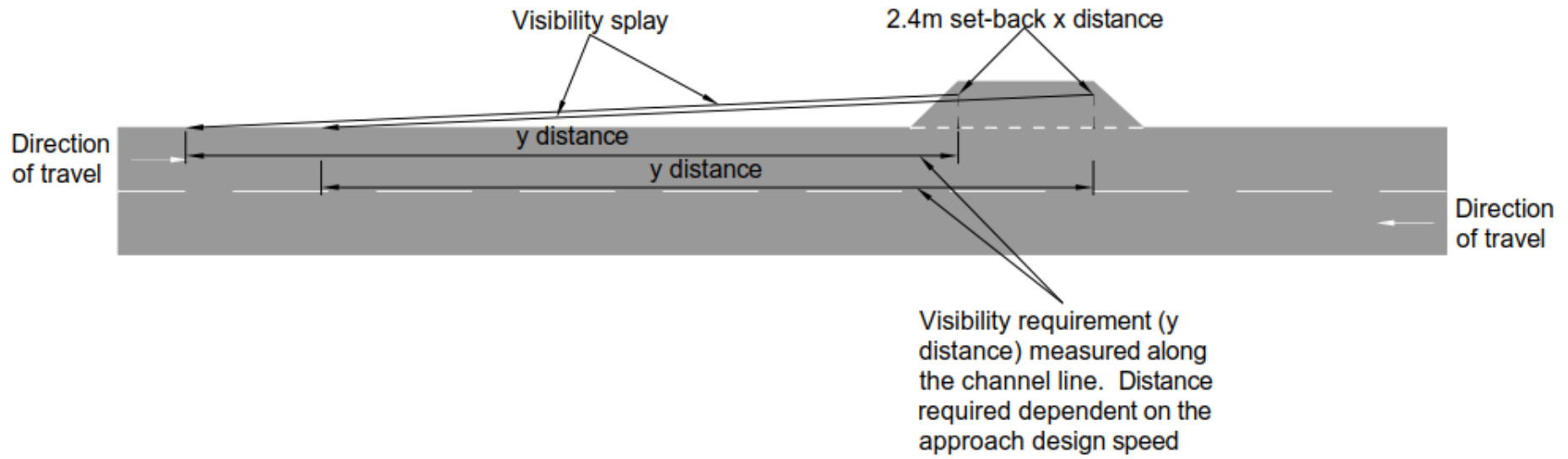
Figure 3.17Na Visibility requirements at the exit from a type B parking lay-by - nearside lane
