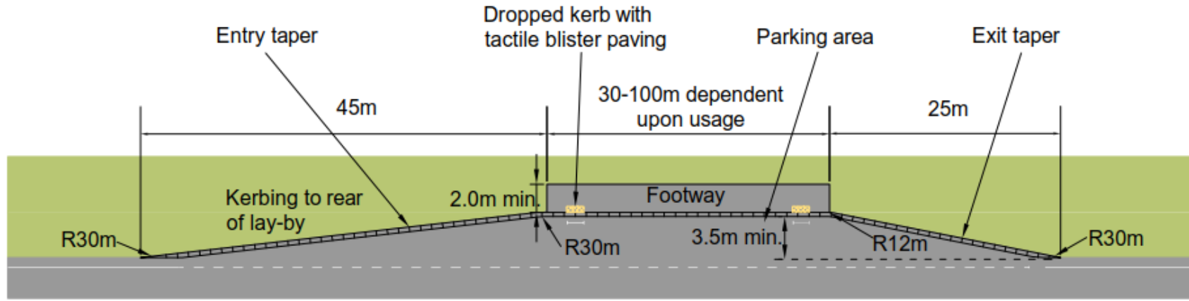
Figure 4.30N Geometric layout of type B lay-by (to be used only on single carriageway roads with speed limits not exceeding 40 mph)
